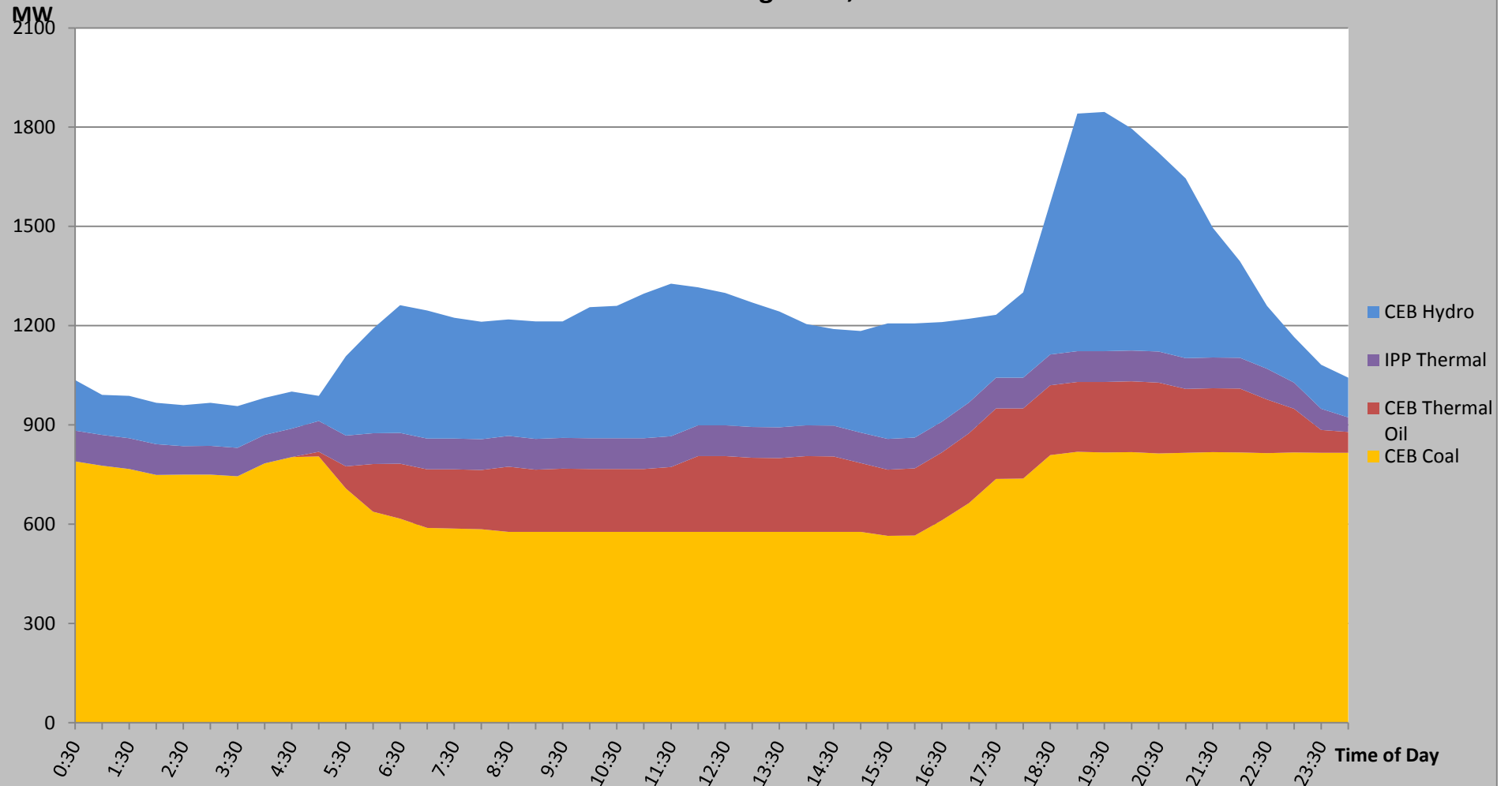
Load Curve for August 28, 2016
