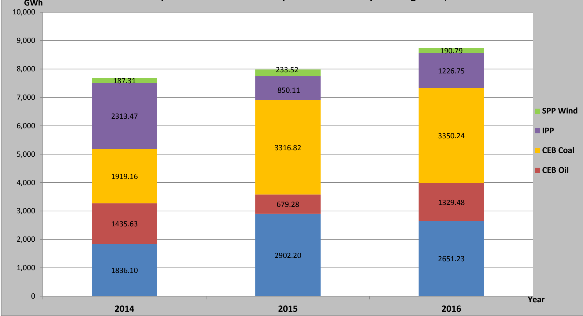
Comparison of Cumulative Dispatch from January 1 to August 29, 2016
