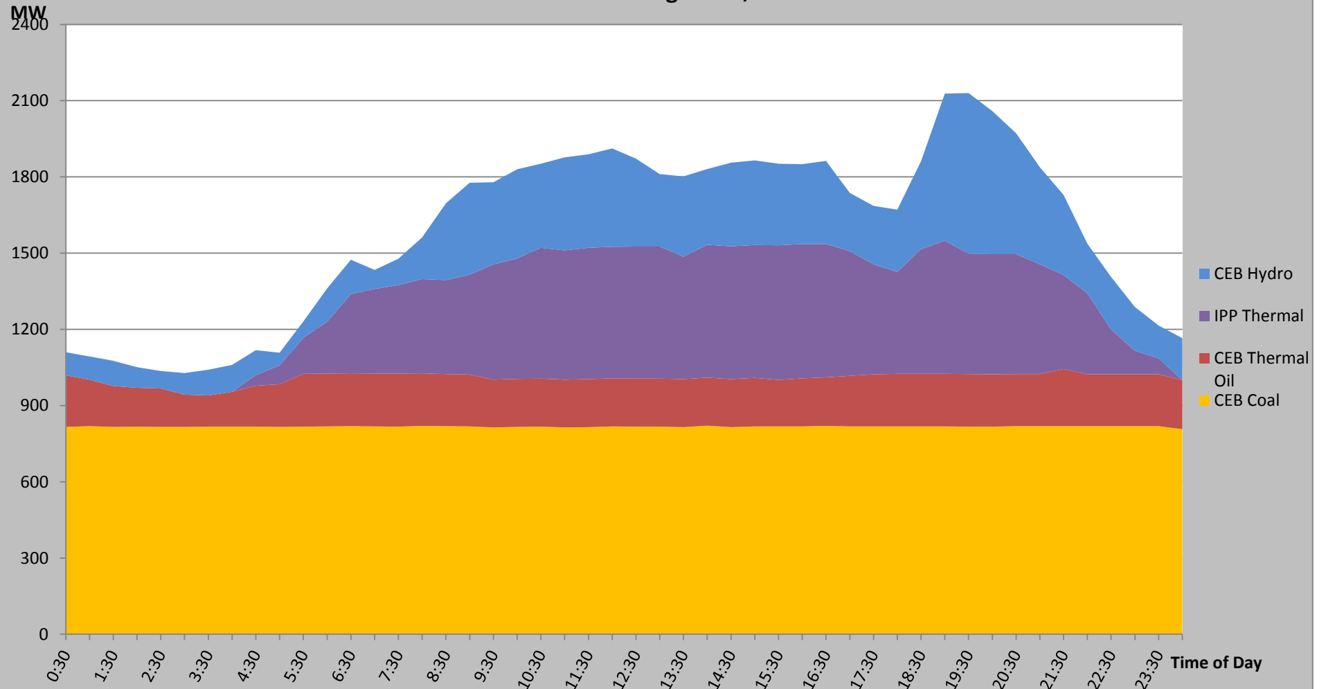
Load Curve for August 25, 2016
