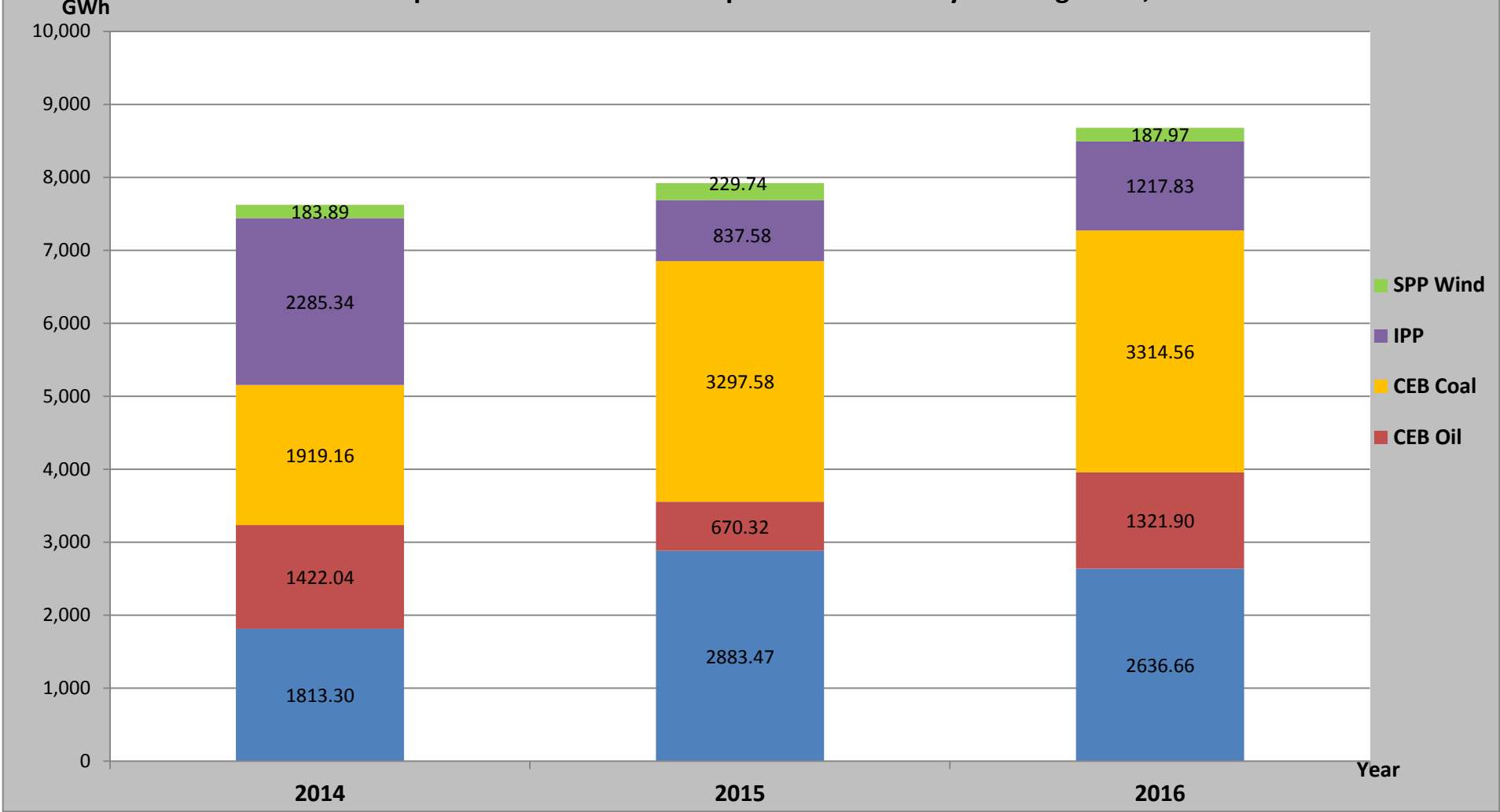
Comparison of Cumulative Dispatch from January 1 to August 27, 2016
