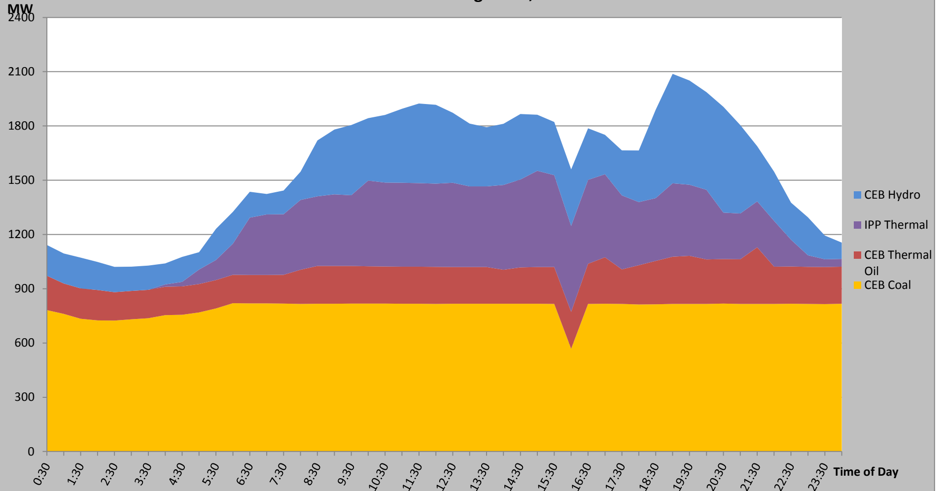
Load Curve for August 26,2016
