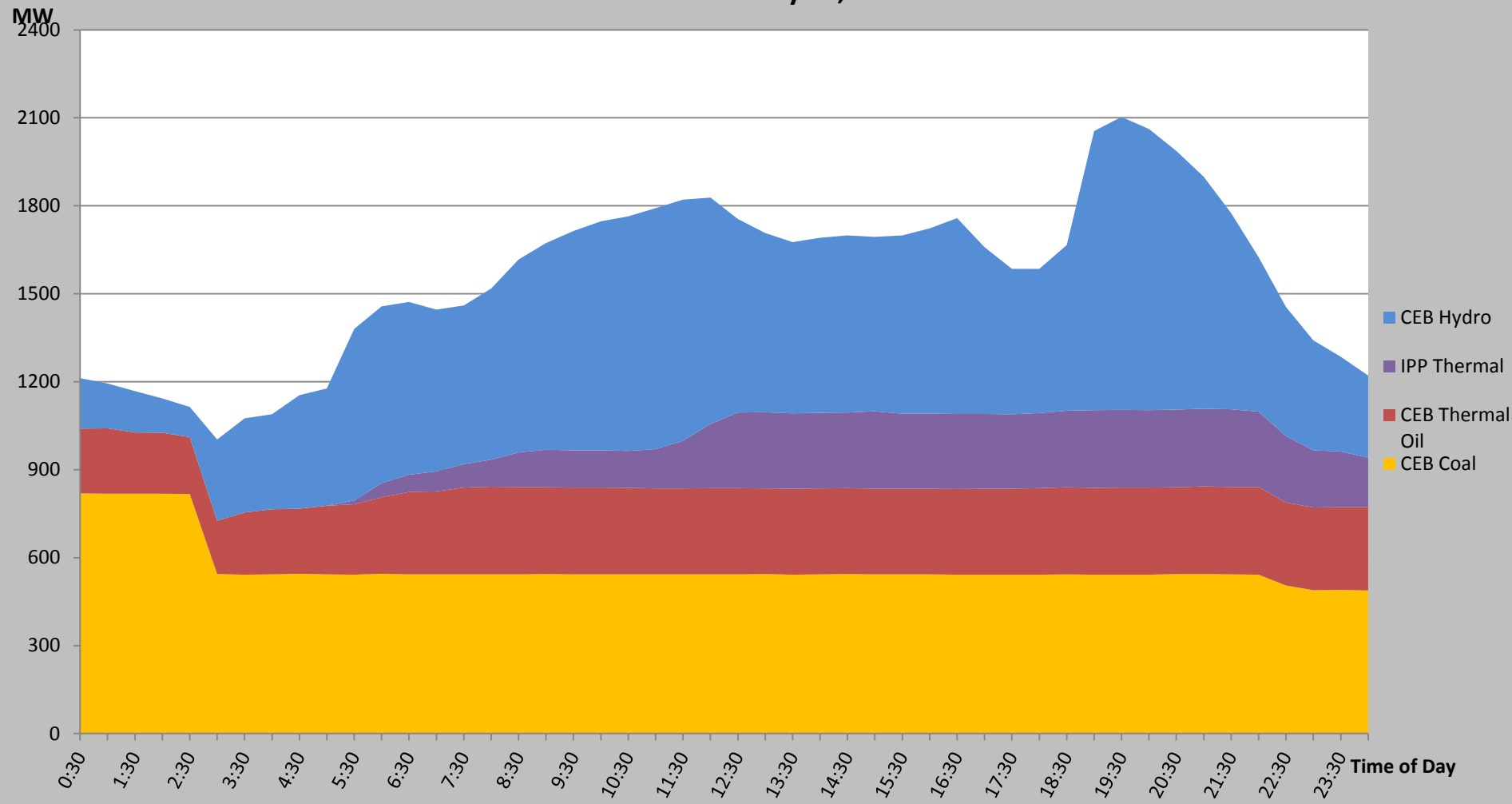
Load Curve for July 06,2016
